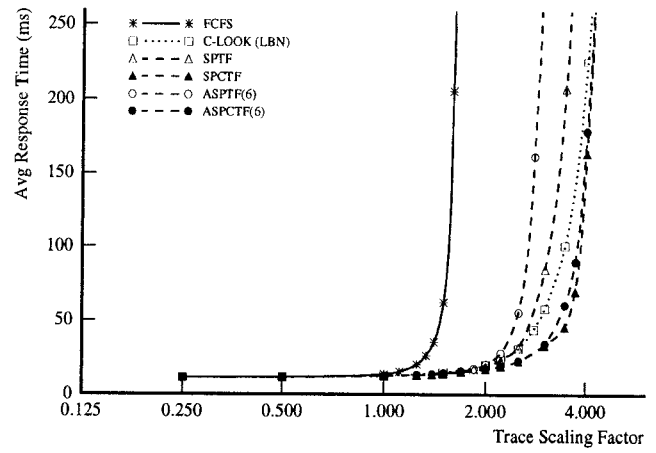
Figure 13: Full-Knowledge Scheduling of Sci-TS
