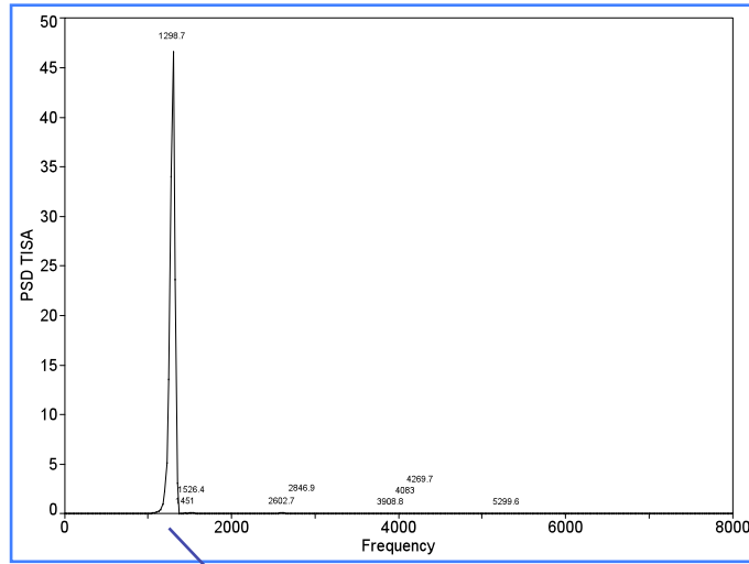
Power spectral density of the impact window
