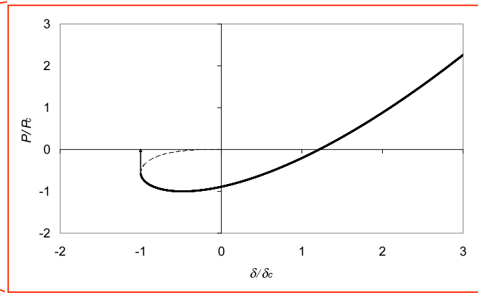
Load-deflection characteristics for one asperity
