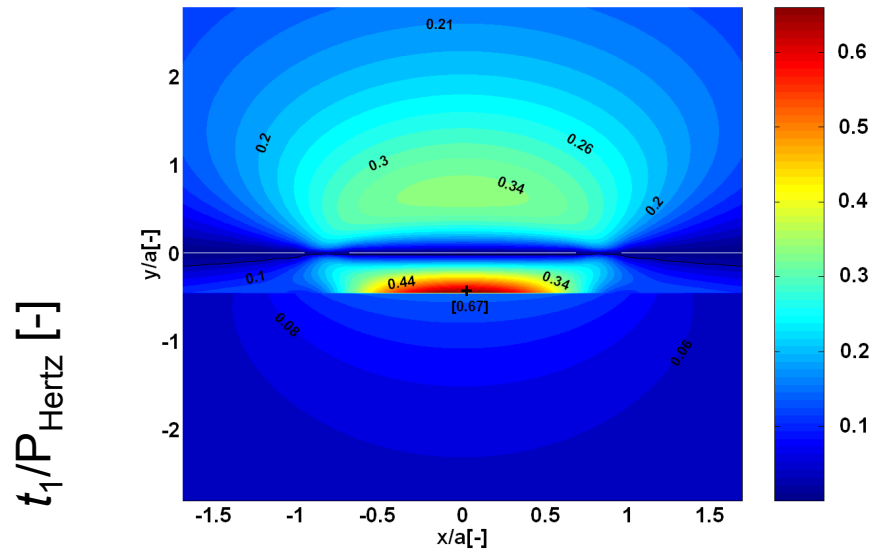
Sub-surface stress field for a tappet coated with a layer of 5mm DLC
