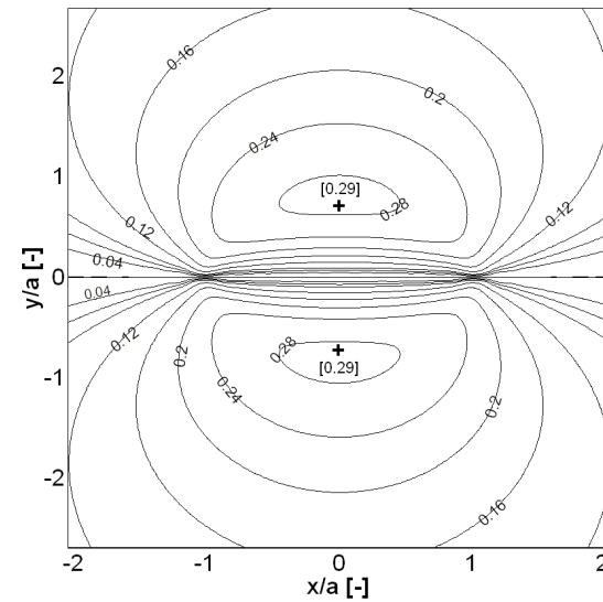
Sub-surface stress field for an uncoated tappet
