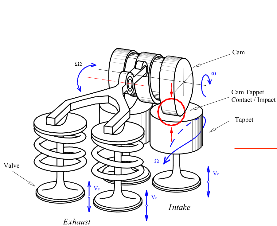
Single Cylinder bike engine (Honda CR 450)
