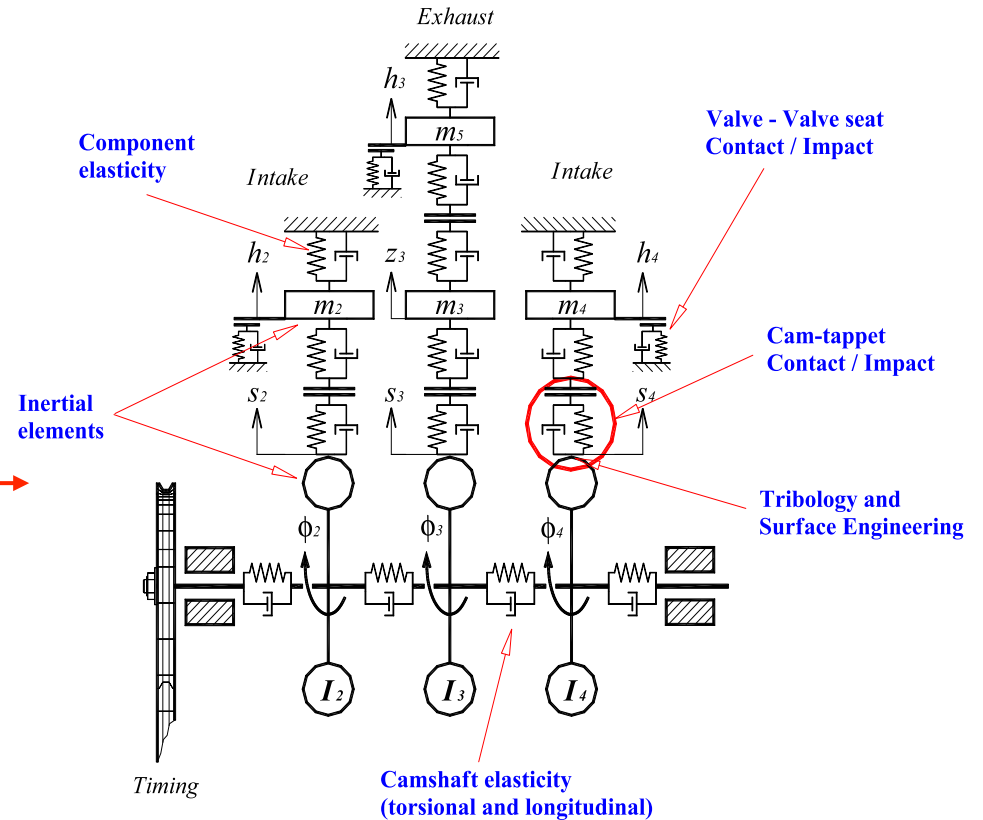
Single Cylinder bike engine (Honda CR 450)
