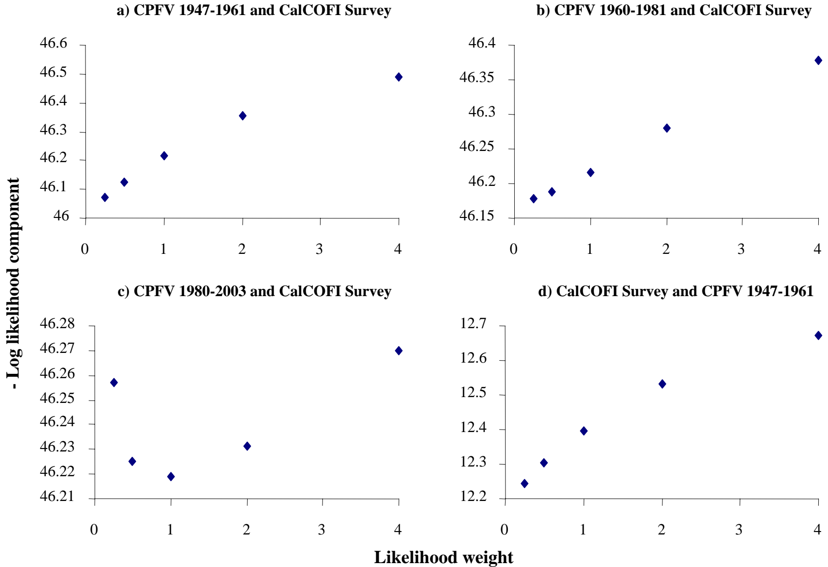
Figure 6.22 a-d We varied the likelihood weight of each of the four surveys individually while holding all other likelihood weights at the baseline level at one. In each panel, the likelihood component of one survey is shown as another survey's likelihood weight is varied. We focus on comparing the CPFV surveys with the CalCOFI survey.
