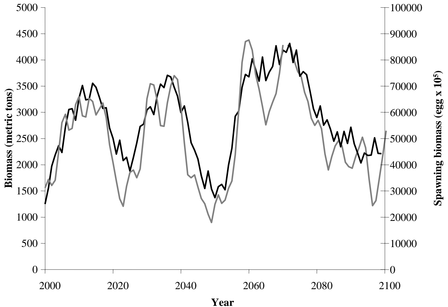
Figure 7.4 Variable recruitment leads to temporal variation in expected total and spawning biomass even in the absence of fishing mortality. The results presented here are based on a single projection showing for total (black line) and female (grey line) spawning biomass in the absence of fishing assuming that recruitment is selected randomly from model estimated recruitment from 1970-1995.
