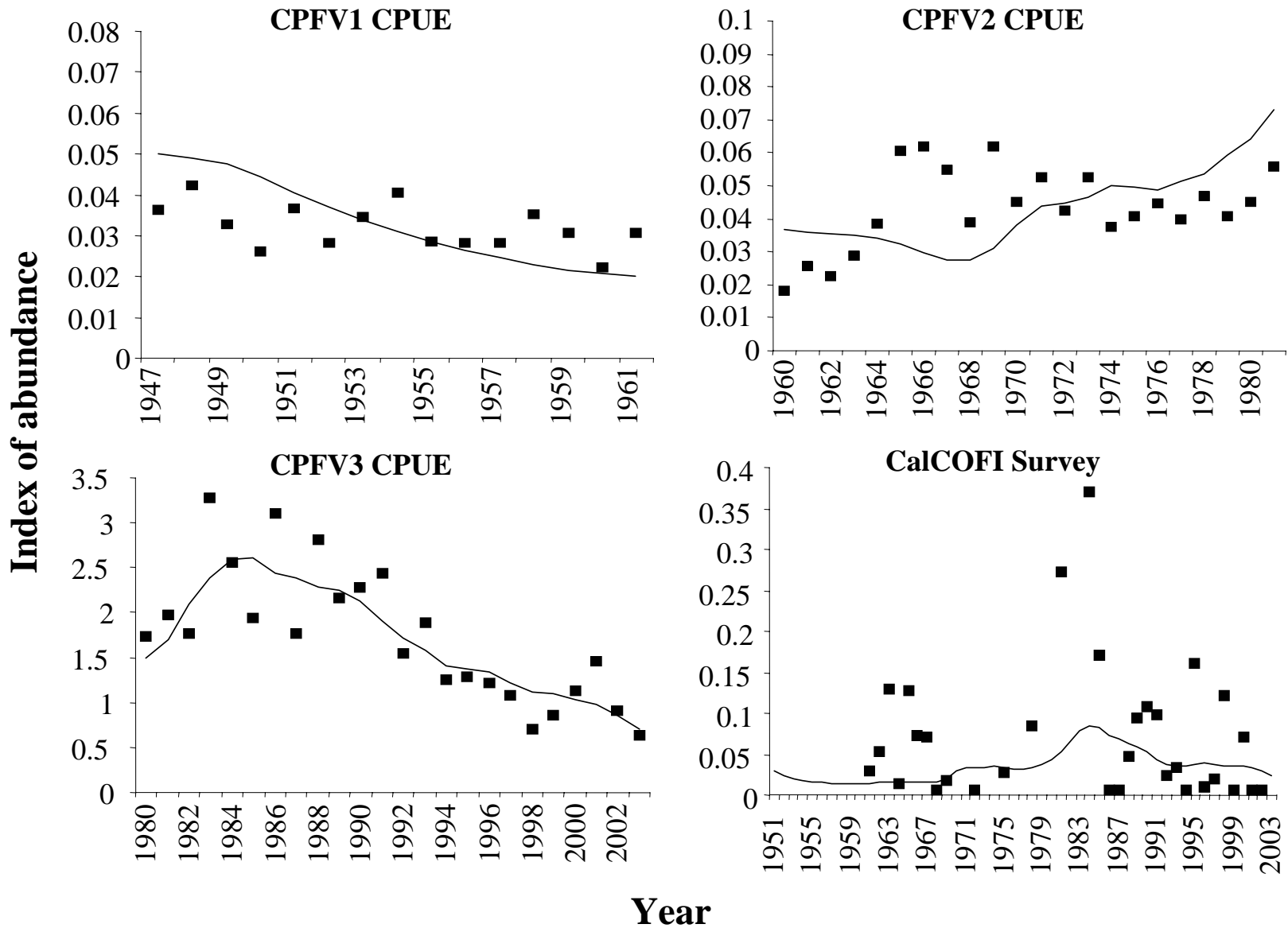
Figure 8.7 The estimated (solid line) and observed (black squares) abundance indices for the final Synthesis model when M=0.15 .
