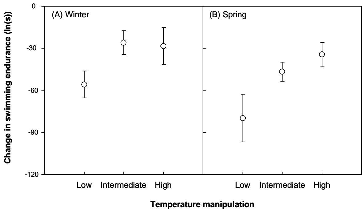
FIG. 2.3 Change (Mean \pm SE) in swimming endurance (sec) of three-spined sticklebacks over the breeding season in relation to temperature treatment (low, intermediate and high); in two separate experiments temperatures were manipulated for four weeks in either (A) the Winter or (B) the Spring prior to the breeding season. Data are expressed as in Fig. 2.2; negative values indicate that swimming endurance was poorer at the end of the breeding season. See text for analyses.
