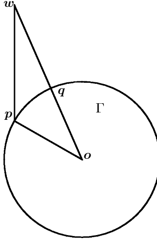
Figure 2: Illustration for the proof of Theorem 5
