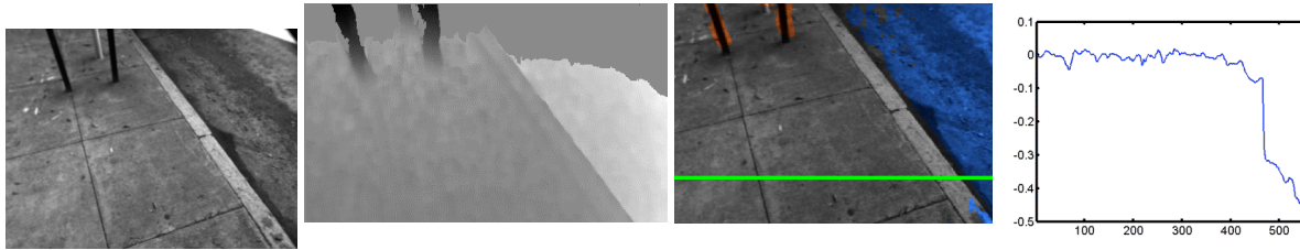
Figure 1. Stereo input and output. Left to right: (a) Image from left camera. (b) Elevation map (darker = higher). (c) Areas classified as above (red), below (blue) and on (no color) ground plane. (d) Graph of elevation across the green slice in panel (c) is roughly constant except for the discontinuity at the curb.
