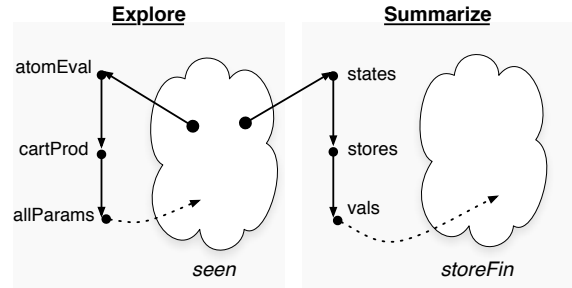
Figure 5. Simplified handler network for k -CFA. Exploration and summarization processes are driven by the same LVar. The triply-nested forEach calls in summarize become a chain of three handlers.
