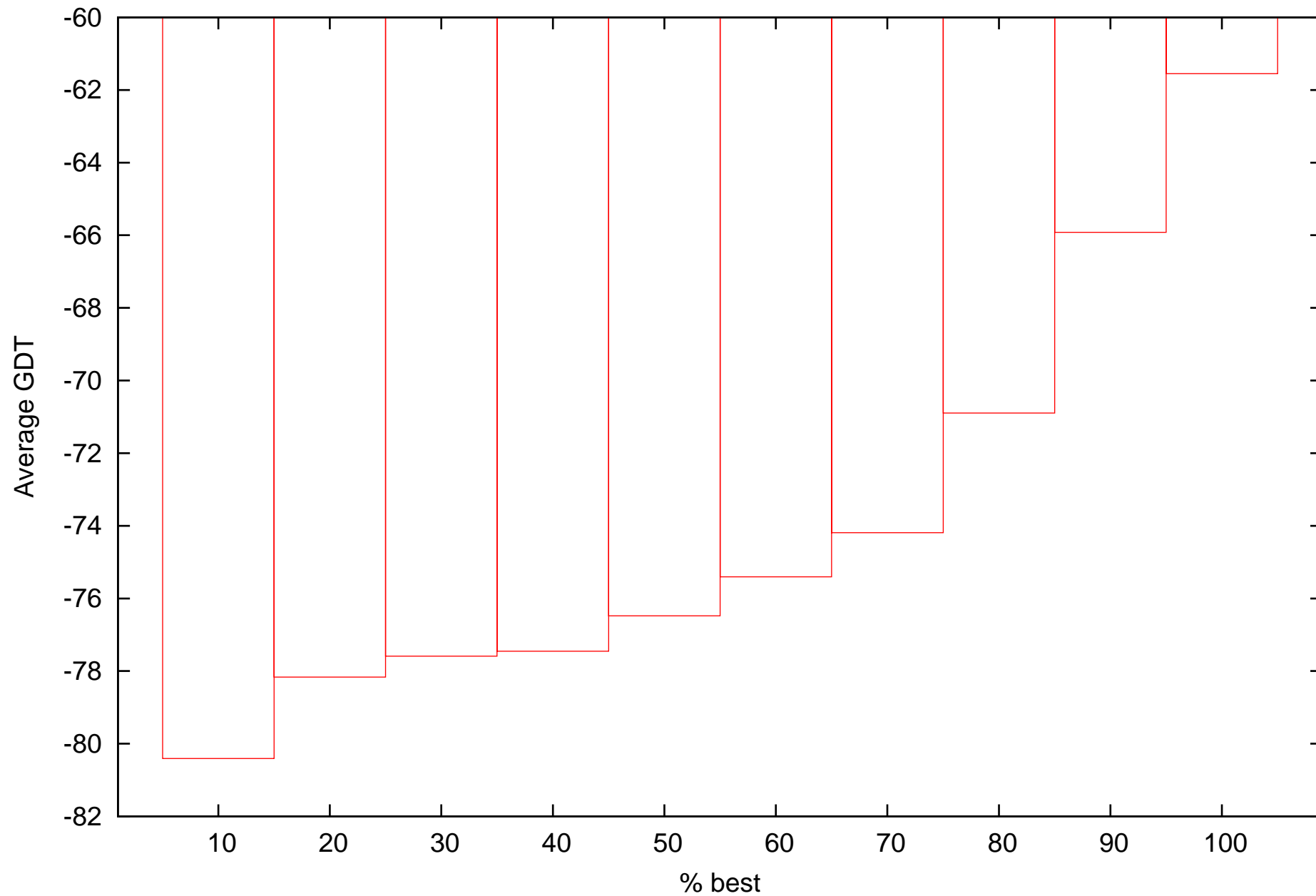
T0367 constraint-optimized_bonus_nonc-1.1.costfcn
