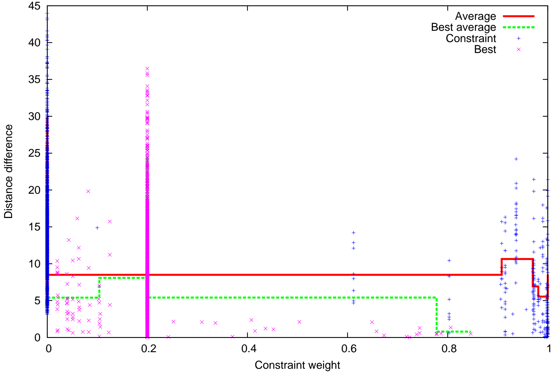
T0348 constraint-best.costfcn
