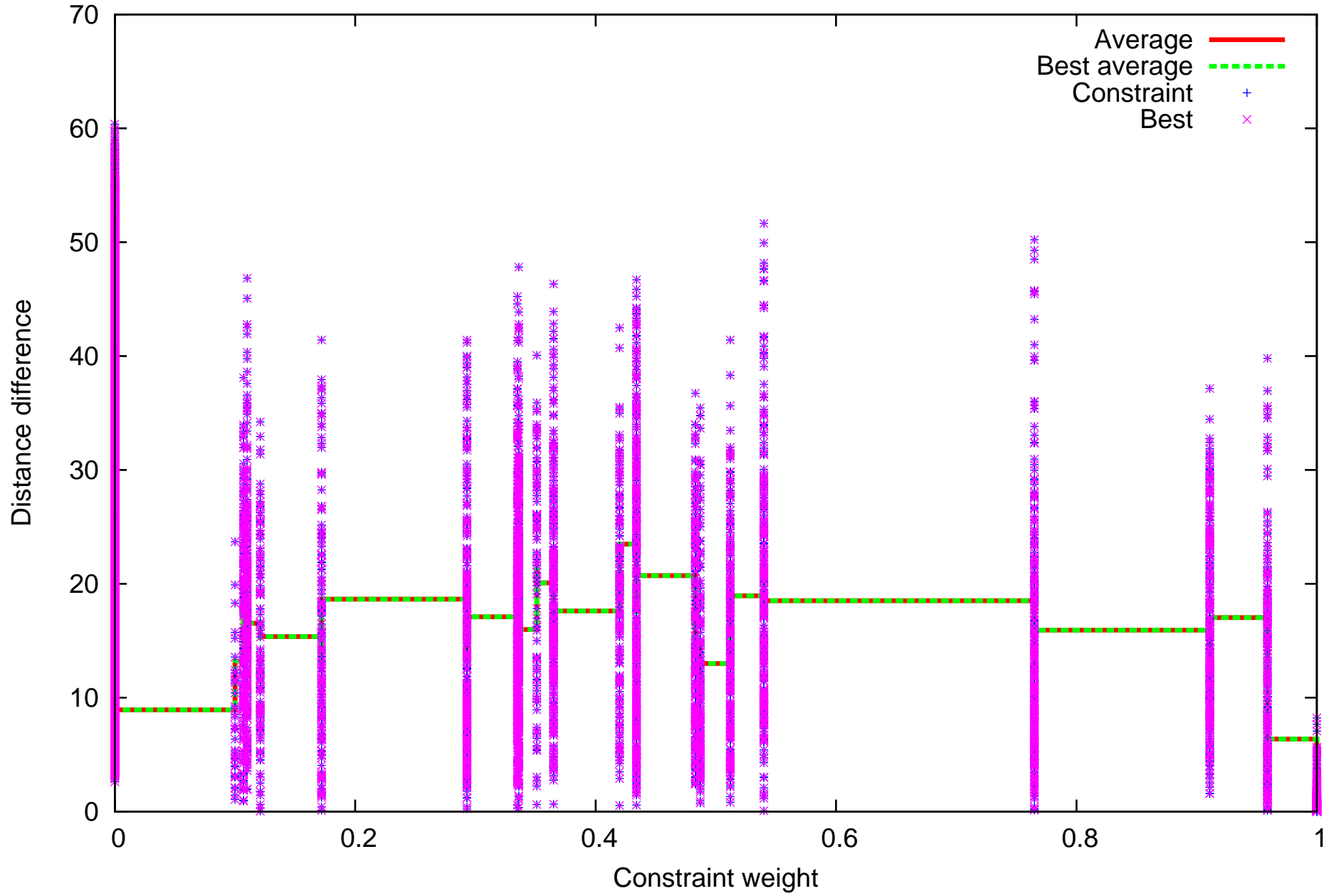
T0328 alignment_constraints-good-all.under
