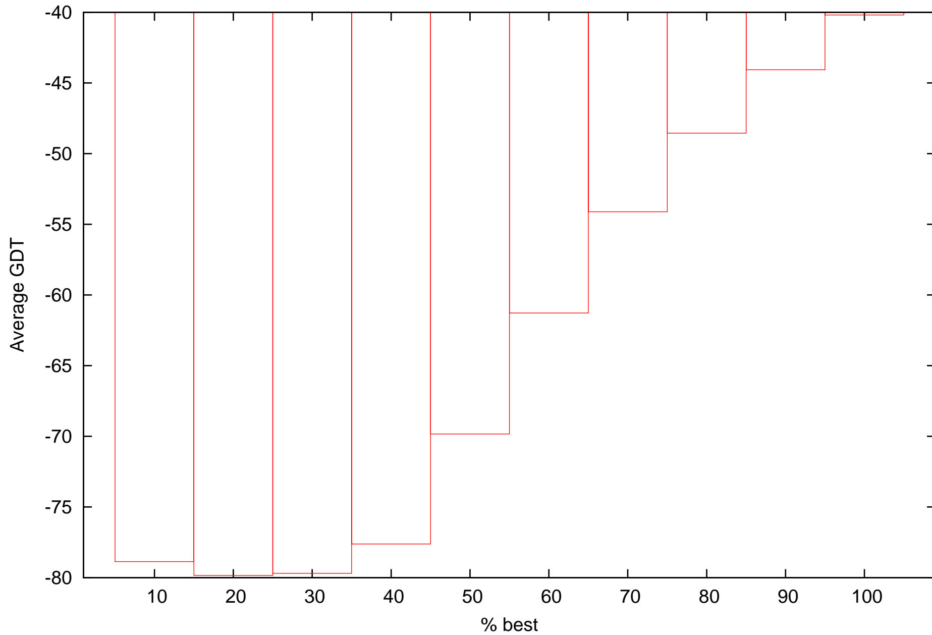
T0328 alignment_constraints-good-all-8.under
