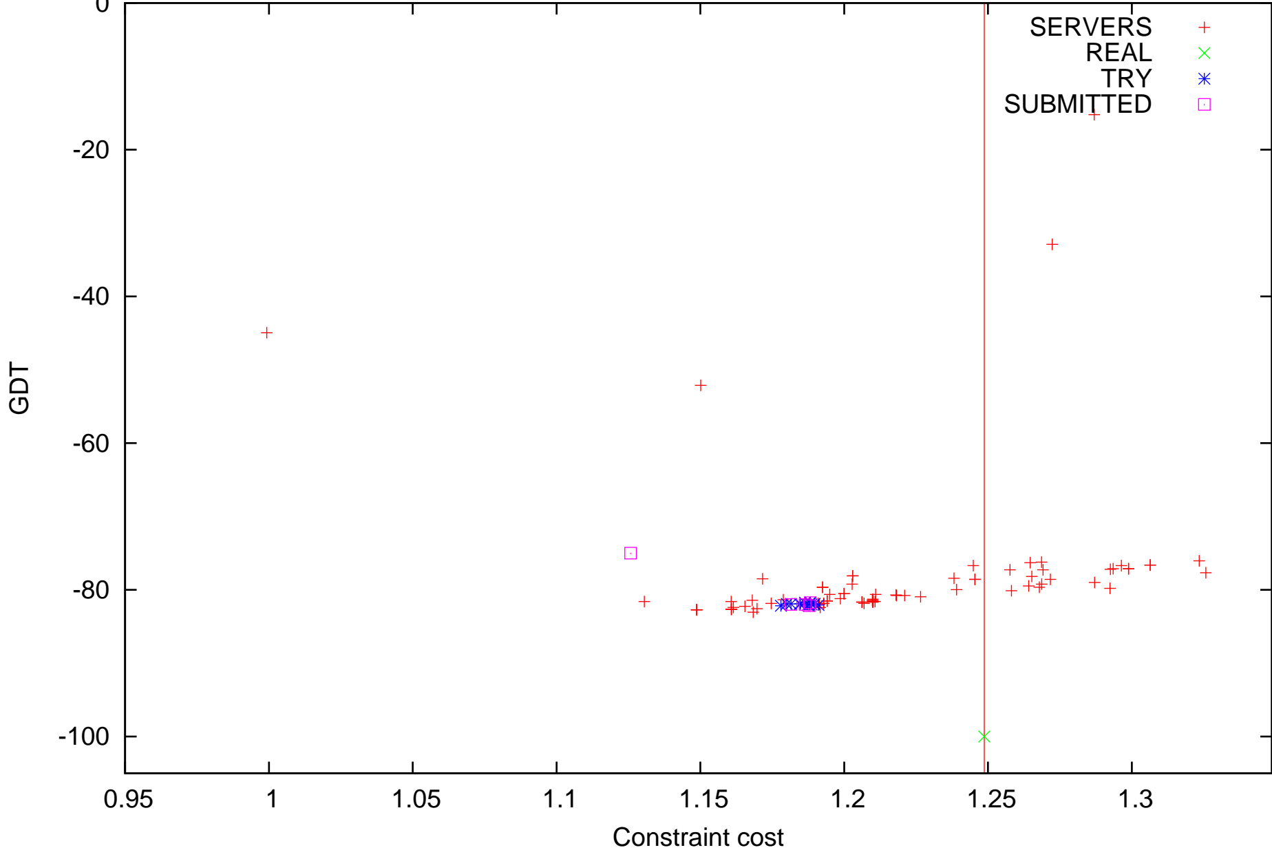
T0328 alignment_constraints-good-all-8.under
