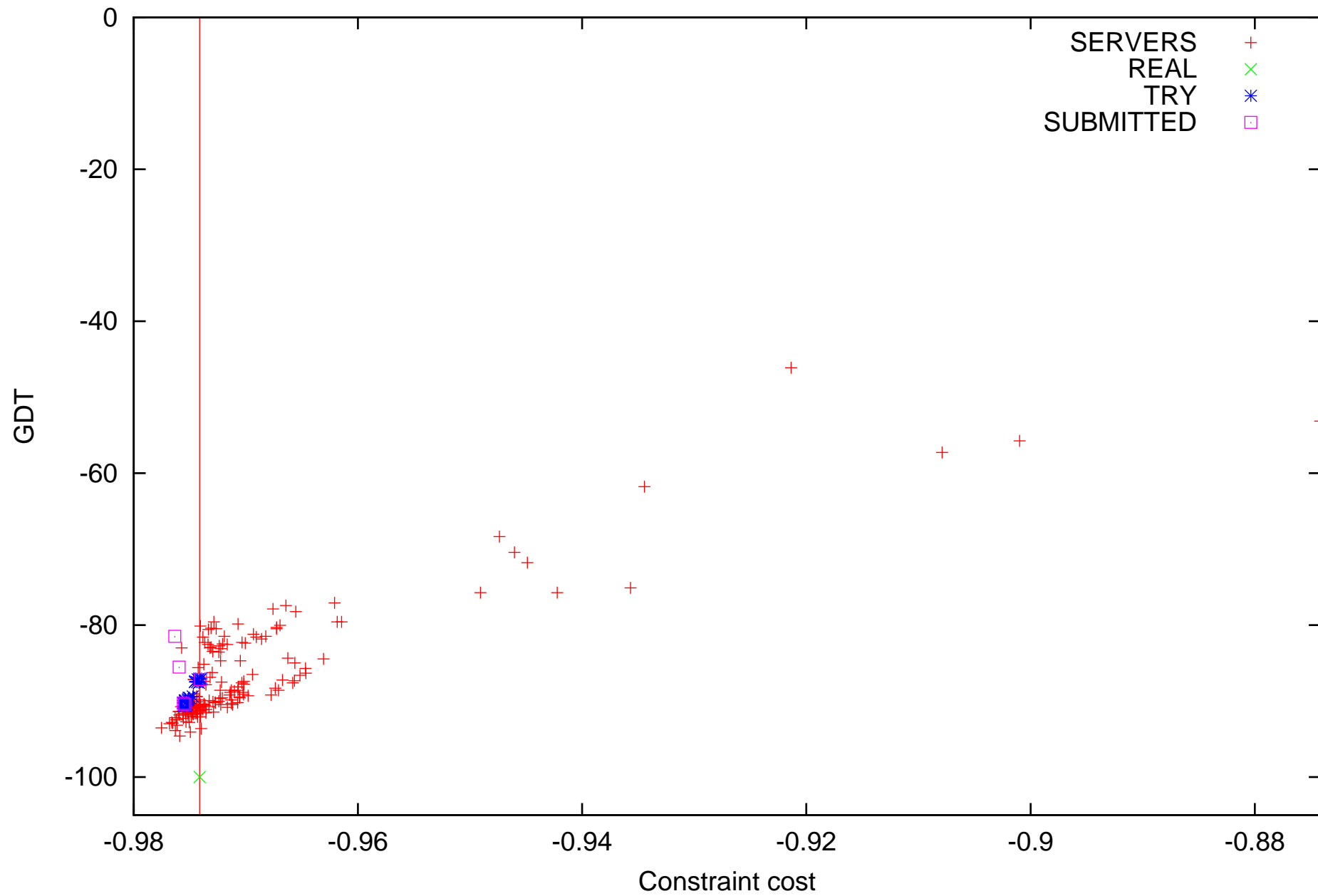
T0305 constraint-optimized_bonus_nonc-1.1.costfcn
