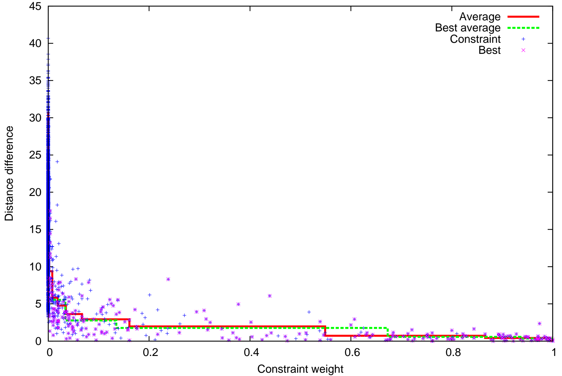
T0288 constraint-optimized-0.6.costfcn
