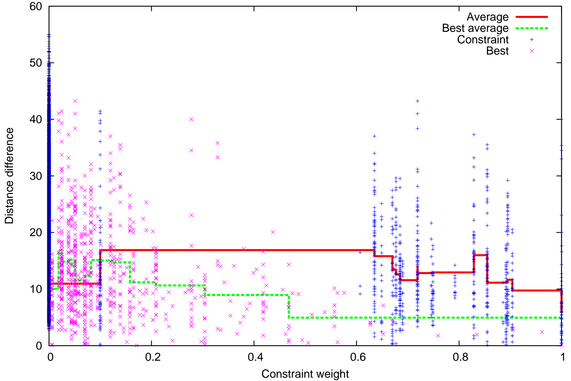
T0283 constraint-fraction-good-all100.costfcn
