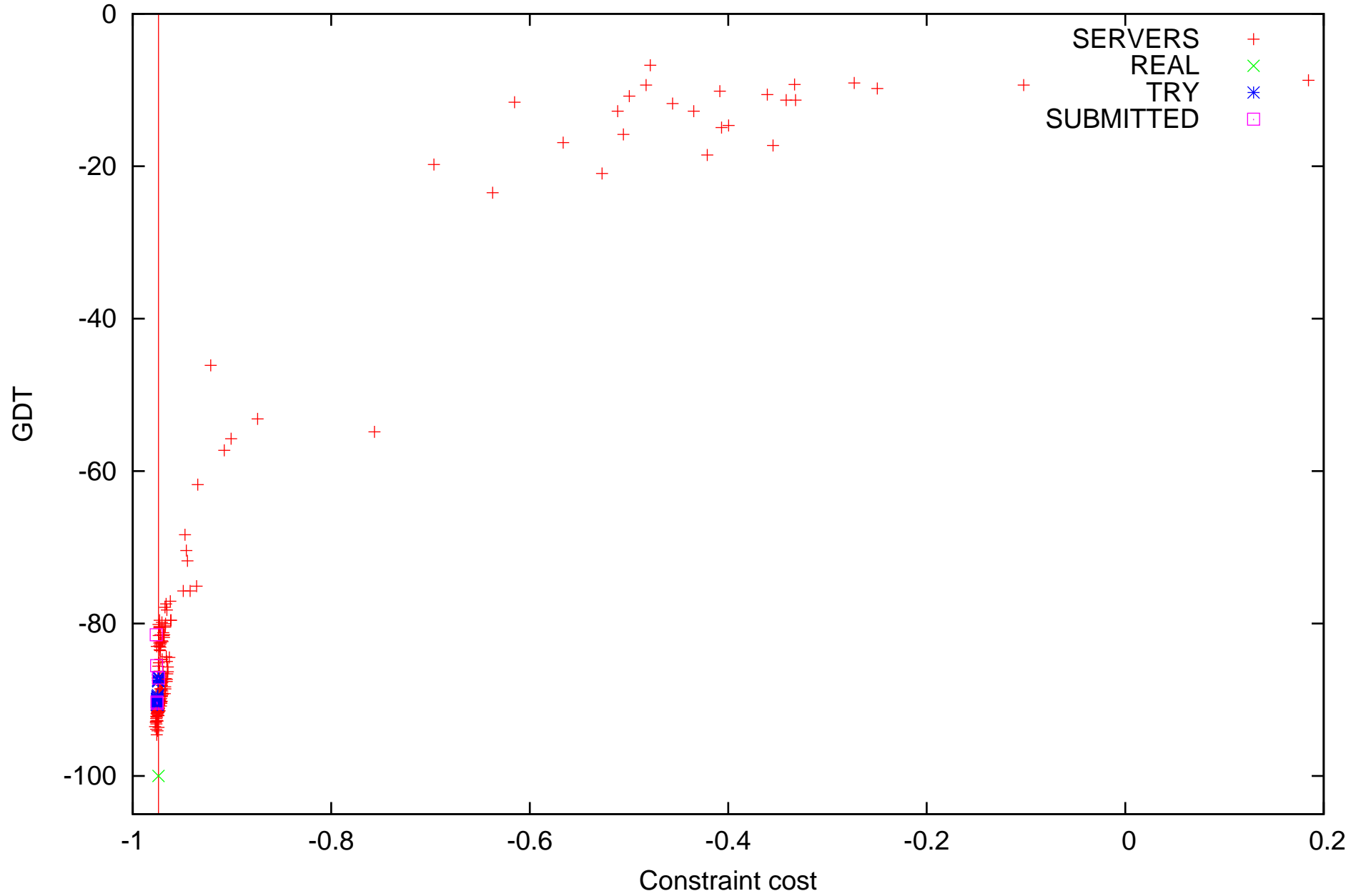
T0305 constraint-optimized_bonus_nonc-1.1.costfcn
