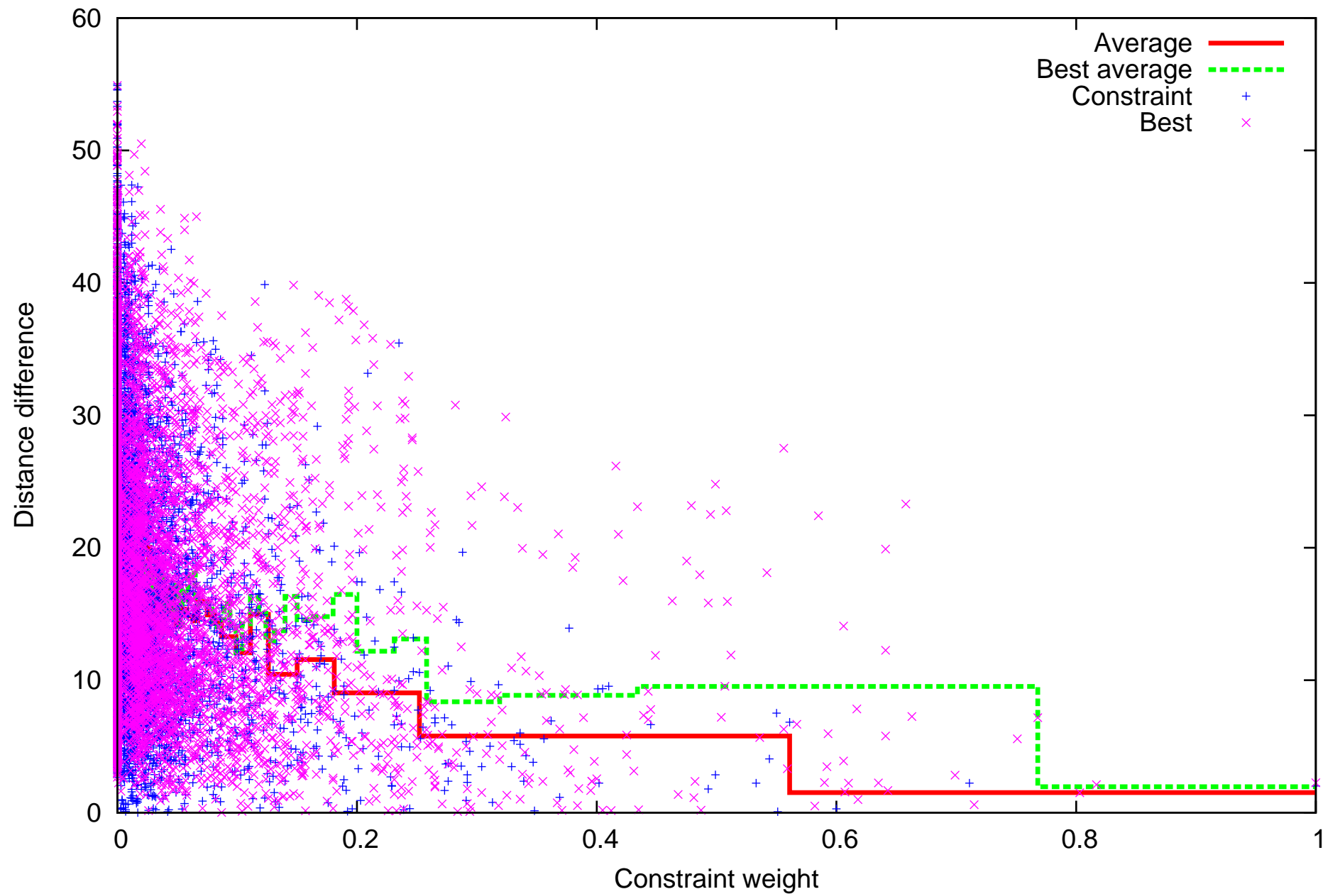
T0283 constraint-meta-0.costfcn
