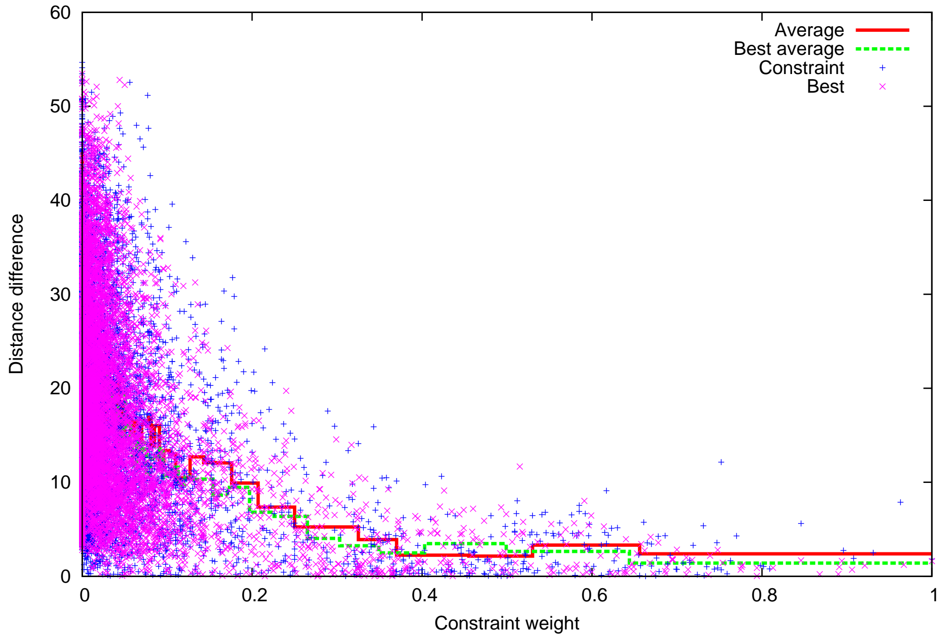
T0383 constraints-combined.under
