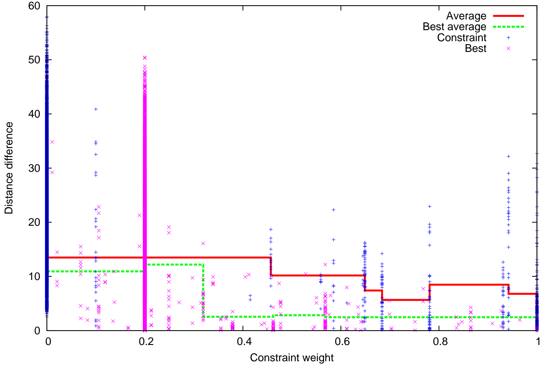
T0383 constraint-best.costfcn
