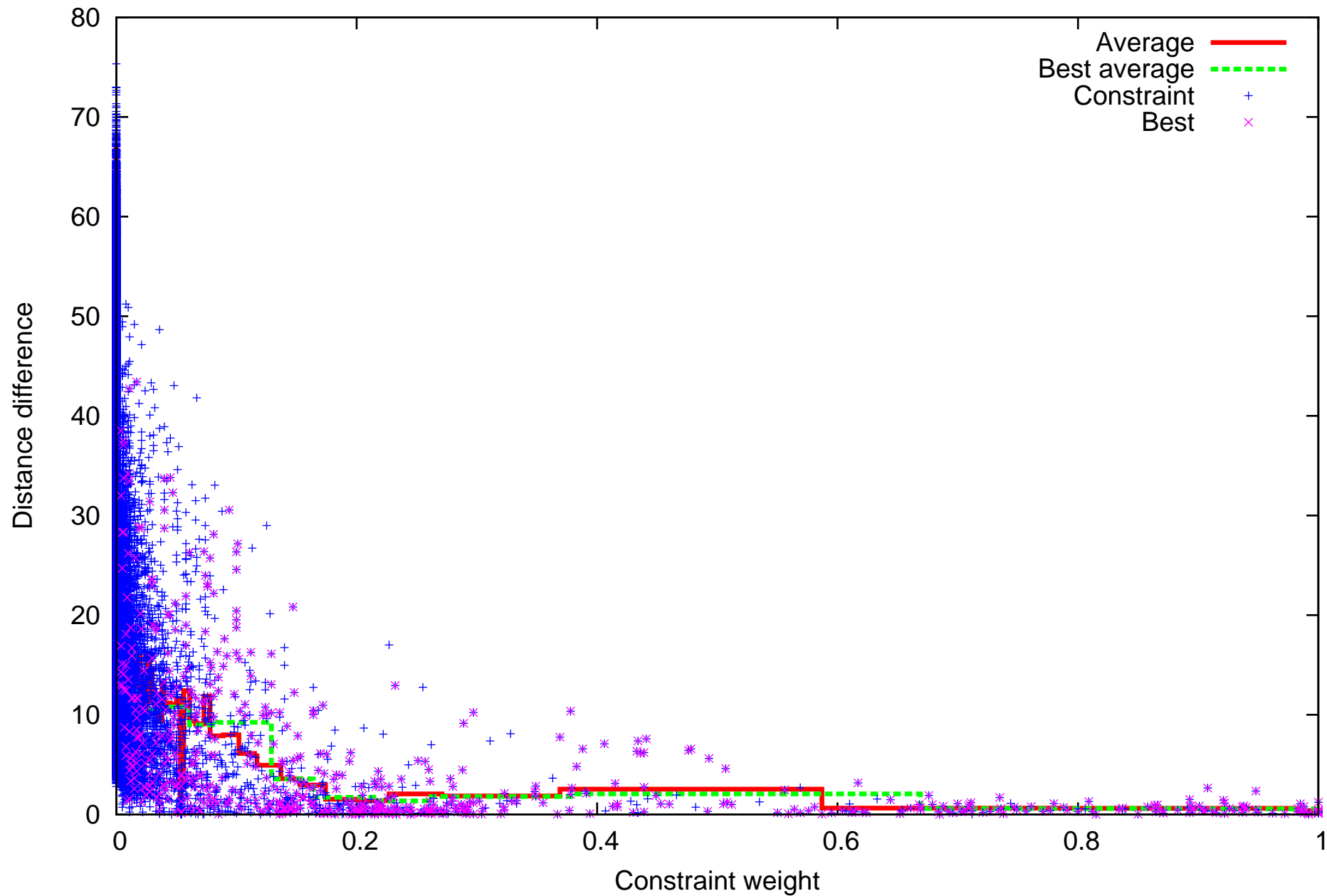
T0295 constraint-optimized-0.6.costfcn
