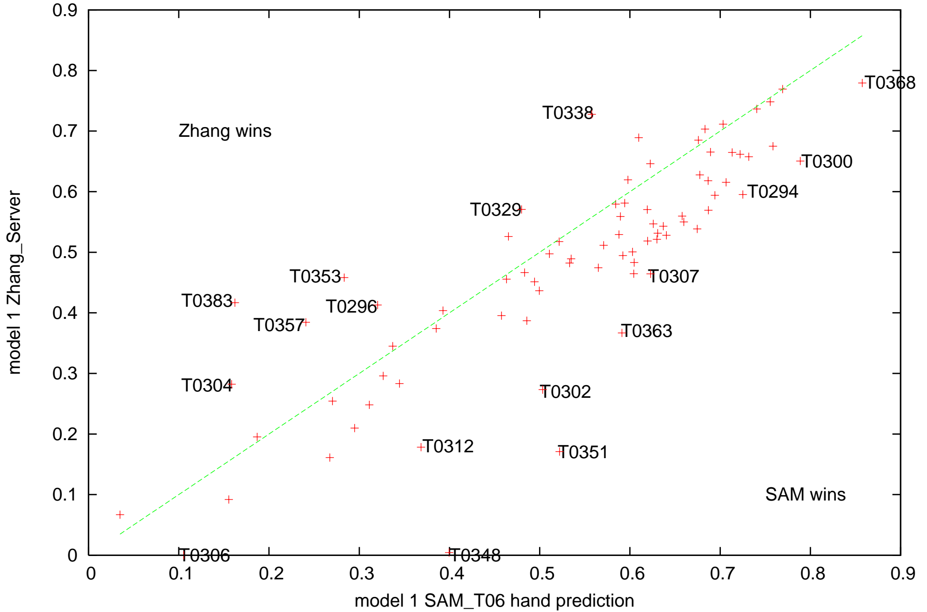
real_hbond comparison (1.0 is best)
