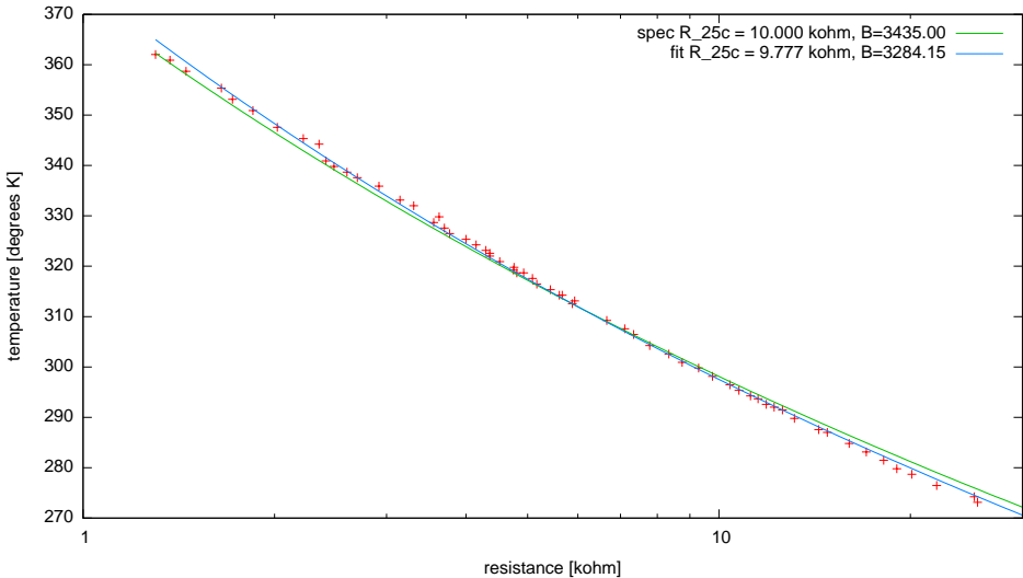
Thermistor NTCLE413E2103F520L
