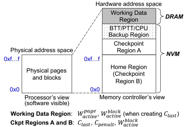
Figure 4: ThyNVM address space layout.
