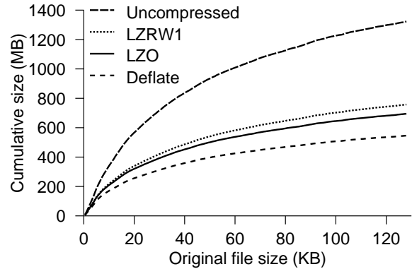
Figure 6. Cumulative space required for compressed files.
