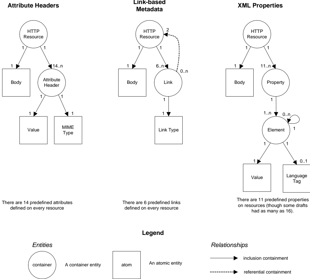
Figure 2 – Containment models of WebDAV metadata designs.
