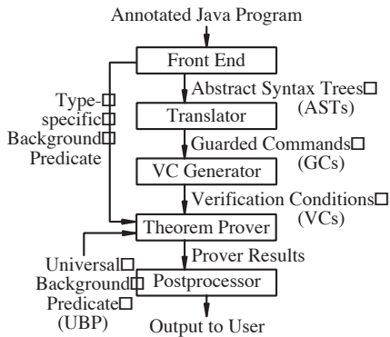
Figure 3: The basic steps in ESC/Java’s operation.
