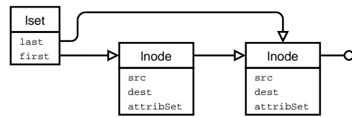
Figure 3: A set of links from a file in AnonFS
