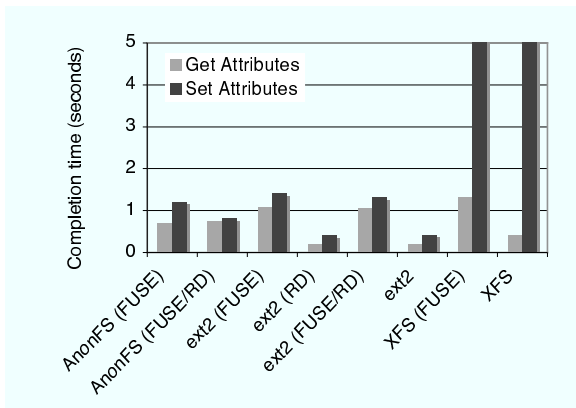
(a) Setting and getting file attributes on 15,620 files ( k = 5 , d = 5 , n = 4 , a = 2 ). The times are in seconds and averaged over 5 runs. RD indicates file system on RAM-disk. Note that the XFS runs to set attributes both took over 21 seconds; the graph is cut off at 5 seconds to show details for the other runs.
