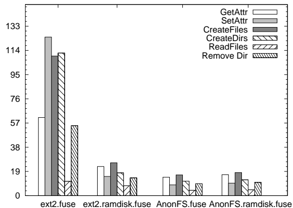
Figure 11: Running times of the 6 file system operations for ext2 and AnonFS through FUSE. Results are averaged over 4 runs on a 111,110 directory tree with 1 zero-byte file per directory ( k = 10 , d = 6 , n = 1 ).
