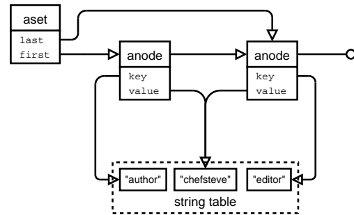
Figure 4: A set of attributes in AnonFS
