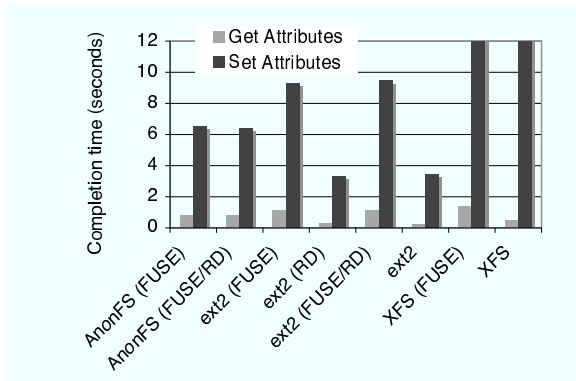
(b) Setting and getting file attributes on 15,620 files ( k = 5 , d = 5 , n = 4 , a = 20 ). The times are in seconds and averaged over 5 runs. RD indicates file system on RAM-disk. Again, XFS, both with and without FUSE, was much slower, requiring over 109 seconds to complete the set attributes benchmark. The graph was cut off to show detail for the other file systems.
