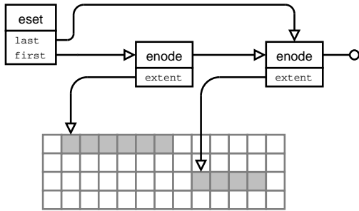
Figure 5: AnonFS extent system for disk allocation
