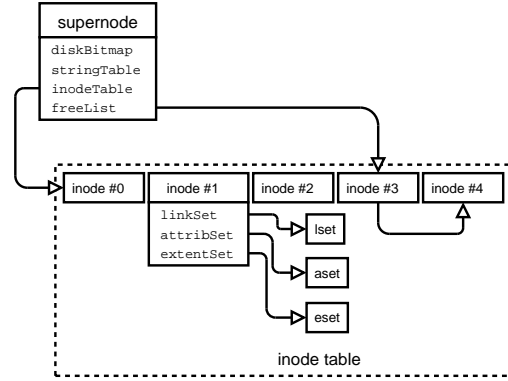
Figure 2: Structure of the AnonFS supernode
