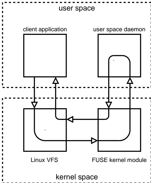
Figure 6: The relationship between FUSE and the FUSE/AnonFS userspace daemon
