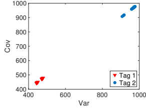
Fig. 11. Example of K-Medoids process. Two tags in a pair can be clustered by comparing the physical-layer features.
