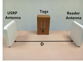
Fig. 4. System Deployment
