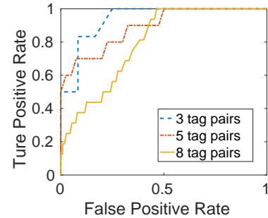
Fig. 29. The ROC curve of multiple tag-pairs
