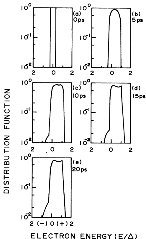
FIG. 3. Time evolution of the distribution function in the field of 1 \times 10^4 V/m with the zero-field Fermi energy of 0.3\Delta , showing electron confinement in the region below \Delta ; the distribution functions (a) at 0 ps, (b) at 5 ps, (c) at 10 ps, (d) at 15 ps, and (e) at 20 ps.
