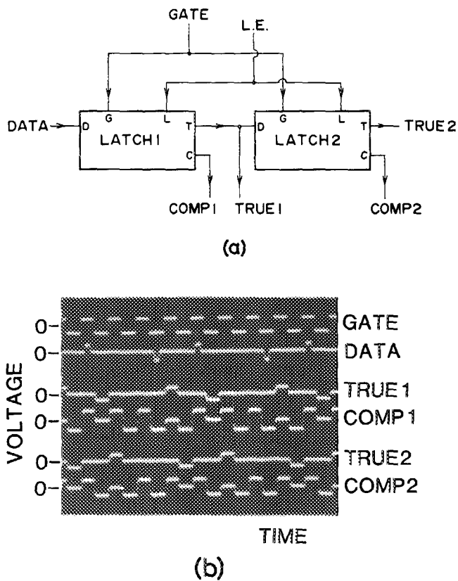
FIG. 5. The two-bit serial latch experiments. GATE, DATA, and TRUE (COMP) 1,2, represent power supply current, input data to the 1st latch, and the true (complement) output of the 1st or 2nd latch, respectively. The true output is generated only when the data-signal "1" is applied during the last cycle, while the complement output is generated only when the data signal "0" is applied during the last cycle. The proper data transfer from latch to latch is shown. (a) The schematic circuit diagram of the experiments. (b) The operation photograph of the two-bit latch with true and complement outputs.
