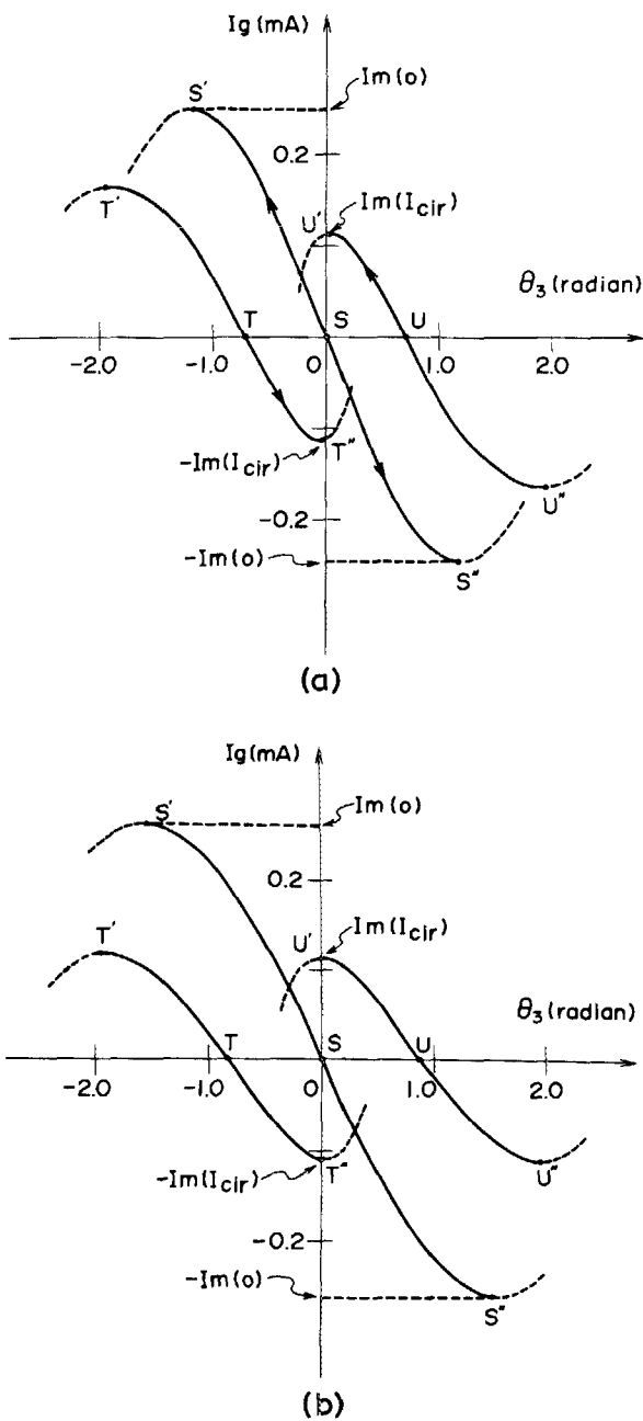
FIG. 3. The characteristics of the sense gate Q_1 having a storage loop calculated using measured circuit parameters: (a) in the presence of a parasitic inductance and (b) in the absence of a parasitic inductance. The threshold gate current I_g is plotted as a function of the quantum phase difference \theta_3 of the junction J_3 . The solid lines represent the thermodynamically stable regions and the broken lines represent the unstable regions.
