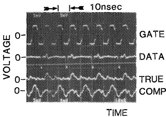
FIG. 7. The high-speed operation of a latch at 6-ns cycle time. GATE, DATA, TRUE, and COMP represent power supply current, data signal, true and complement outputs, respectively. The input data sequence 0, 0, 1, 0 is applied to the latch. The true output 0, 0, 0, 1 and the complement output 1, 1, 1, 0 are generated.
