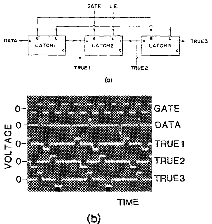
FIG. 6. The three-bit serial latch experiments. GATE, DATA, and TRUE1-3 represent power supply current, input data to the 1st latch, the true outputs of first to the third latch, respectively. The true output is generated only when the data-signal "1" is applied during the last cycle. The proper data transfer from latch to latch is shown. (a) The schematic circuit diagram of the experiments. (b) The operation photograph of the three-bit latch with each true output.
