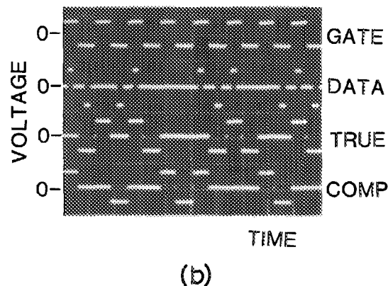
FIG. 4. The one-bit latch experiments. GATE, DATA, TRUE, and COMP represent power supply current, data signal, true and complement outputs, respectively. The latch is powered by a bipolar trapezoidal current. The logical value "0" is represented by a zero-voltage state and the logical value "1" by a voltage state. The true output "1" is generated only when the data-signal "1" is applied during the last cycle, while the complement output "1" is generated only when the data-signal "0" is applied during the last cycle. (a) The schematic circuit diagram of the experiments. (b) The operation photograph of a one-bit latch.
