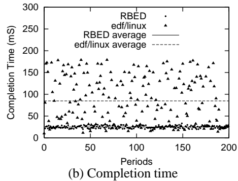
Figure 9: Synthetic best-effort process running with real-time process(190 ms, 150 ms) on RBED and EDF-Linux
