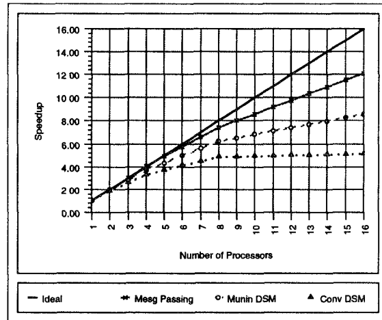
Fig. 12. Gaussian elimination with partial pivoting (GAUSS).
