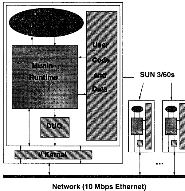
Fig. 5. Munin runtime organization.
