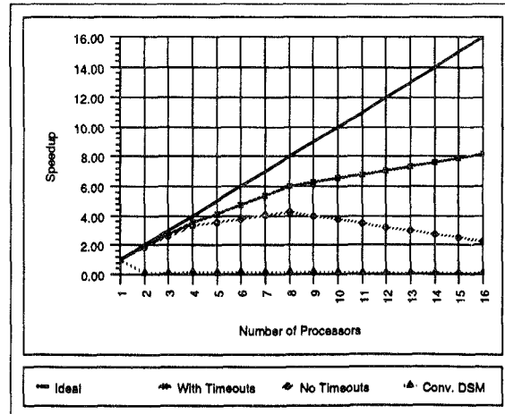
Fig. 17. Effect of update timeout mechanism on FFT.
