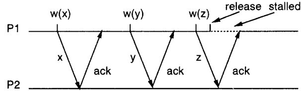
Fig. 1. Pipelining invalidations.
