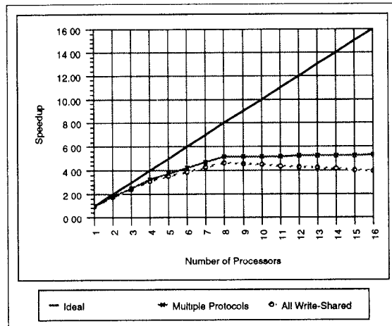
Fig 16. Multiprotocol versus all write-shared (TSP-F).
