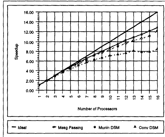
Fig. 7. Finite Differencing (DIFF).
