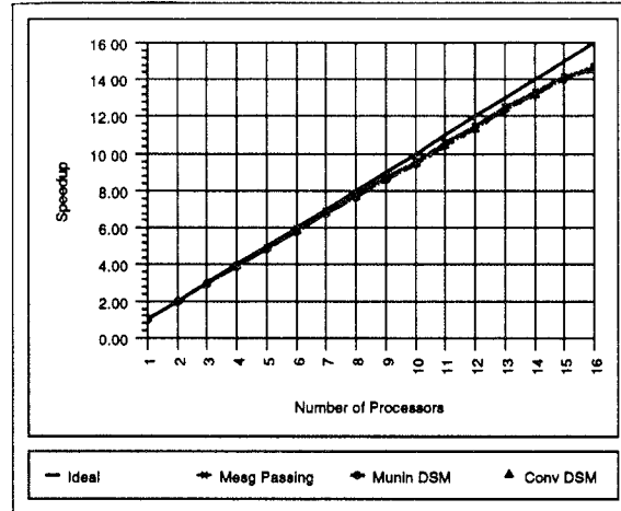
Fig. 6. Matrix Multiplication (MULT).
