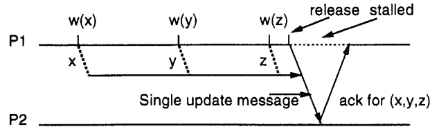
Fig. 2. Buffering and merging updates.
