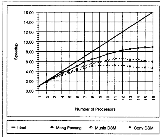
Fig. 9. Fine-grained traveling salesman problem (TSP-F).
