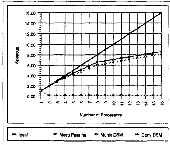
Fig. 11. Fast Fourier Transform (FFT).
