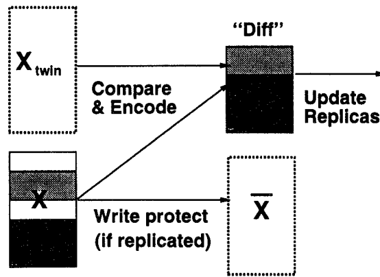
Fig. 4. Write-shared protocol: Sending out diffs .
