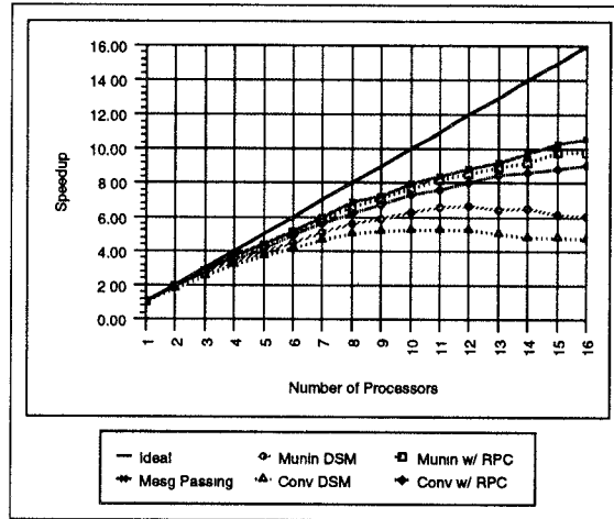
Fig. 18. Effect of function shipping on fine-grained TSP.
