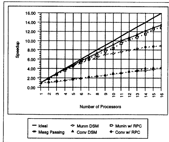
Fig. 19. Effect of function shipping on Quicksort.
