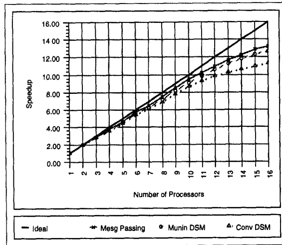
Fig. 8. Coarse-grained traveling salesman problem (TSP-C).
