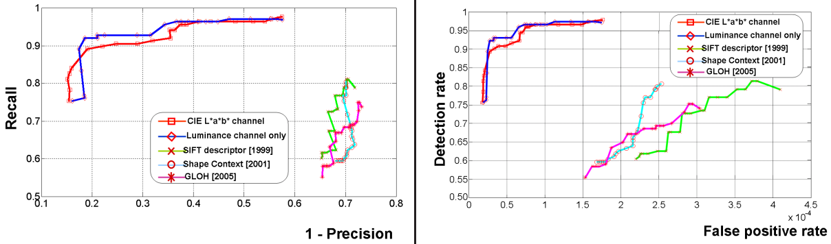
Fig. 24. Left: Comparison of Recall versus 1-Precision curves between luminance channel only and CIE L*a*b* channel on the Shechtman’s test set [7]. It is clearly shown that such descriptors as SIFT [13], GLOH [16], Shape Context [59] turn out to be inferior to LSKs in terms of discriminative power. Right: Comparison of ROC curves. Note that detection rate P_d and false alarm rate P_f are defined as \frac{TP}{nP} ( = recall ) and \frac{FP}{FP+TN} respectively, where TN is the number of true negatives.
