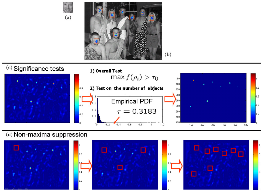
Fig. 9. (a) Query (b) Target with detection (c) Two significance tests (d) Non-maxima suppression [28]
