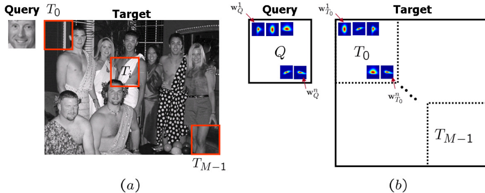
Fig. 2. (a) Given a query image Q , we want to detect/localize objects of interest in a target image T . T is divided into a set of overlapping patches (b) local steering kernels represent the geometric structure of underlying data.
