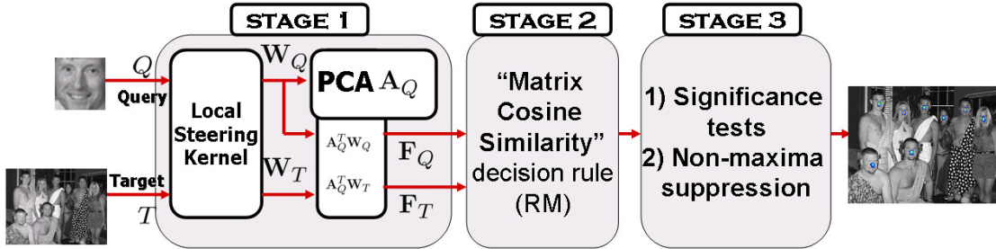
Fig. 1. System overview (There are broadly three stages.)
