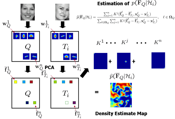
Fig. 10. The estimated conditional density \hat{p}(\bar{\mathbf{F}}_Q | \mathcal{H}_i) is a sum of kernels (weight functions) centered at the features \bar{\mathbf{f}}_{T_i} in T_i which belongs to the hypothesis \mathcal{H}_i . In the Density Estimate Map, red value means a high conditional probability density \hat{p}(\bar{\mathbf{f}}_Q | \mathcal{H}_i) while blue value represents a low conditional probability density \hat{p}(\bar{\mathbf{f}}_Q | \mathcal{H}_i) .
