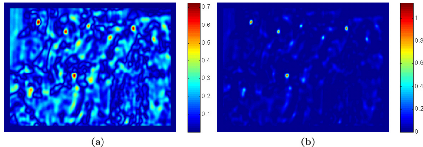
Fig. 7. (a) Resemblance map (RM) which consists of |\rho_i| (b) Resemblance map (RM) which consists of f(\rho_i) . Note that Q and T are the same examples shown in Fig 2.
