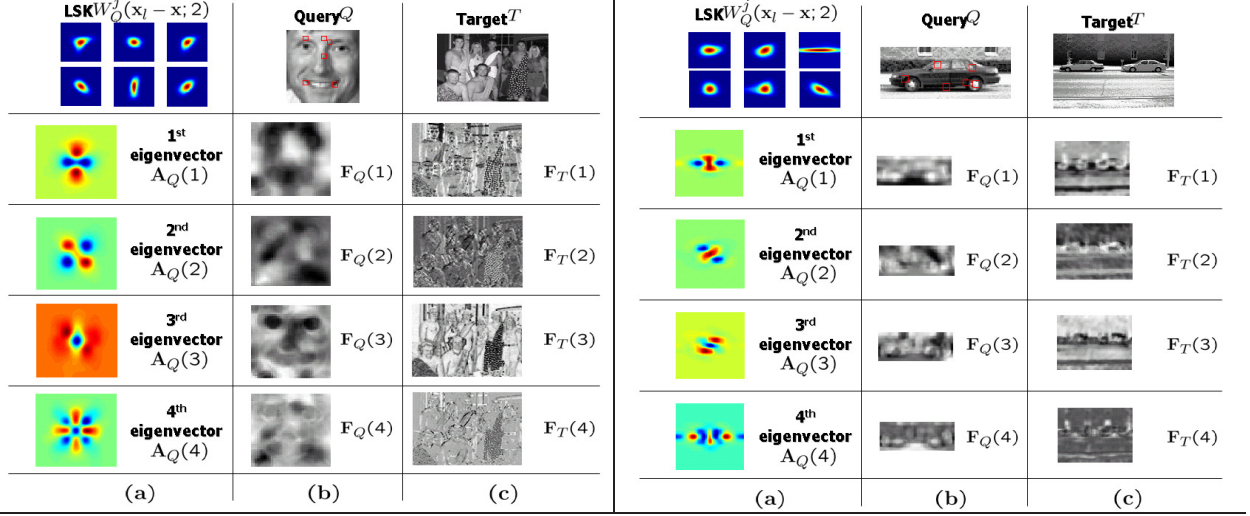
Fig. 6. Face and car examples (a) : \mathbf{A}_Q learned from a collection of LSKs \mathbf{W}_Q , (b): Feature row vectors of \mathbf{F}_Q from query Q , (c) : Feature row vectors \mathbf{F}_T from target image T . Eigenvectors and feature vectors were reshaped into image and up-scaled for illustration purposes.
