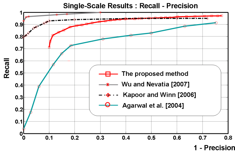
Fig. 15. Comparison of Recall versus 1-Precision curves between the proposed method and state-of-the-art methods [53], [55], [56] on the UIUC single-scale test set [53].
