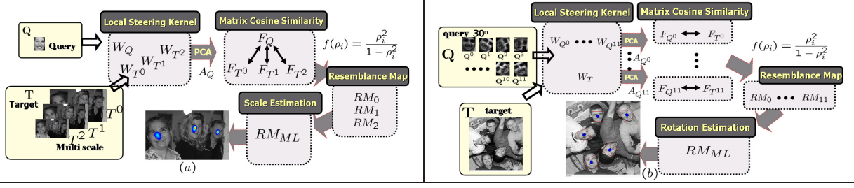
Fig. 12. (a) Block diagram of multi-scale object detection system, (b) Block diagram of multi-rotation object detection system
