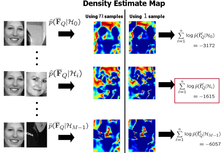
Fig. 11. The estimated conditional probability densities \hat{p}(\bar{\mathbf{F}}_Q|\mathcal{H}_i) using n samples and 1 sample are shown in the middle and the scores on right side means \sum_{\ell=1}^n \log \hat{p}(\bar{\mathbf{f}}_Q^\ell|\mathcal{H}_i) . The higher this score is, the more likely \bar{\mathbf{F}}_Q comes from class i ( \bar{\mathbf{F}}_{T_i} )
