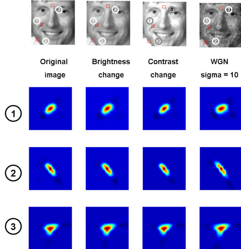
Fig. 4. Invariance and robustness of local steering kernel weights W(\mathbf{x}_l - \mathbf{x}; 2) in various challenging conditions. Note that WGN means White Gaussian Noise.
