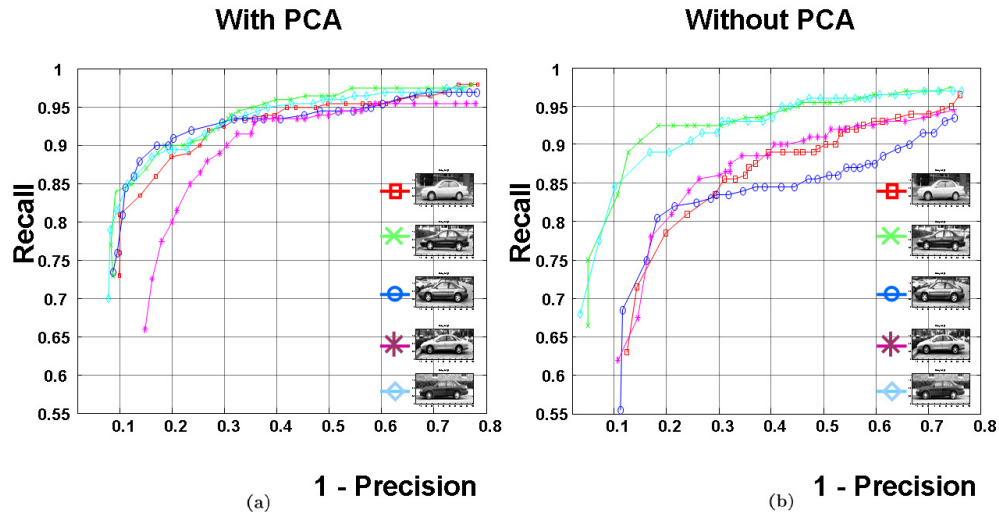
Fig. 14. (a) Recall versus 1-Precision curves of the proposed method (b) Recall versus 1- Precision curves of the proposed method without PCA on the UIUC single-scale car test set [53] using 5 different query images.
