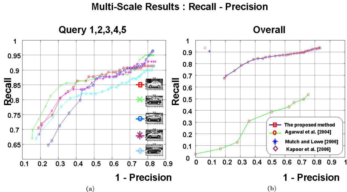
Fig. 16. (a) Recall versus 1-Precisions curve using 5 different query images (b) Comparison of Recall versus 1-Precision curves between the proposed method and state-of-the art methods [56], [57], [53] on the UIUC multi-scale test set [53].
