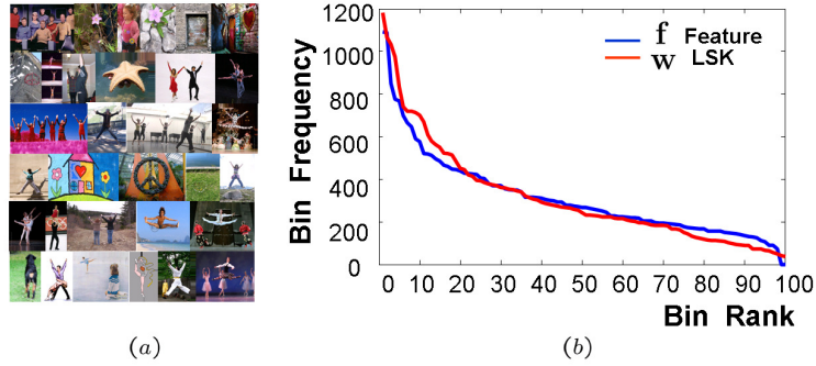
Fig. 5. (a) Some example images (Shechtman’s object dataset [7]) where LSKs were computed. (b) Plots of the bin density of LSKs and their corresponding low-dimensional features.
