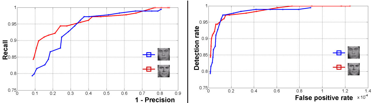
Fig. 20. Left: Precision-Recall curves, Right: ROC curves on the MIT-CMU test set [54] using 2 different query images. Note that detection rate P_d and false alarm rate P_f are defined as \frac{TP}{n_P} ( = recall ) and \frac{FP}{FP+TN} respectively, where TN is the number of true negatives.
