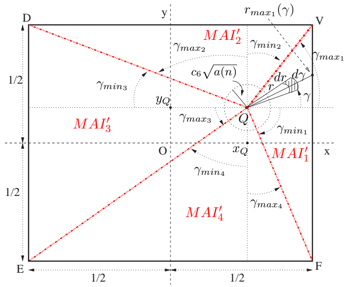
Fig. 6. Interference regions for node i communicating with node j . The angle \gamma increases in the counterclockwise direction.
