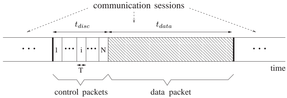
Fig. 5. Time series representation of control and data packets. t_{disc} is the neighbor discovery phase. t_{data} is the time period for transmission of data. t_{disc} plus t_{data} form a communication session.
