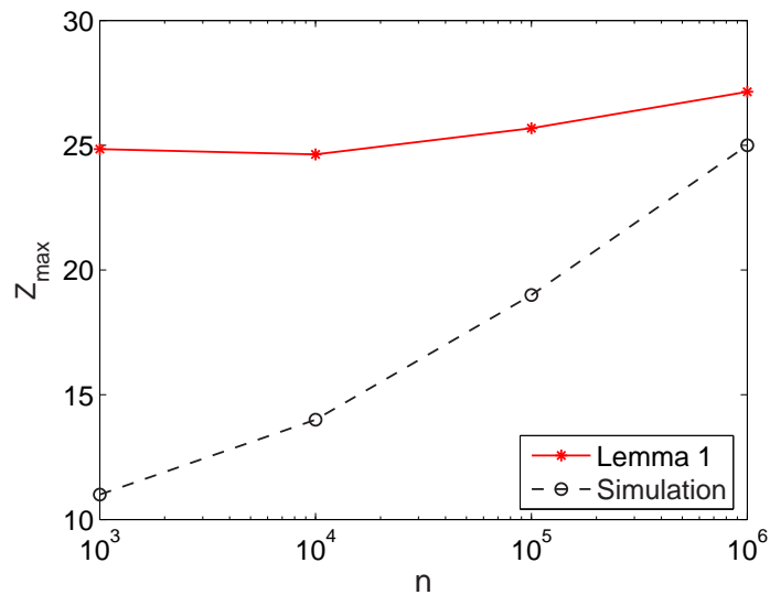
Fig. 1. Maximum number of nodes Z_{max} in a cell as a function of total number of nodes n in the network for \phi = 1/3 from Lemma 1 and from simulations of the uniform mobility model [3].
