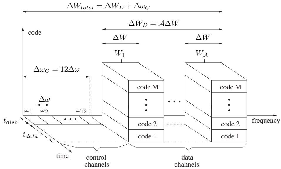
Fig. 3. Data and control channels spectra for the network.
