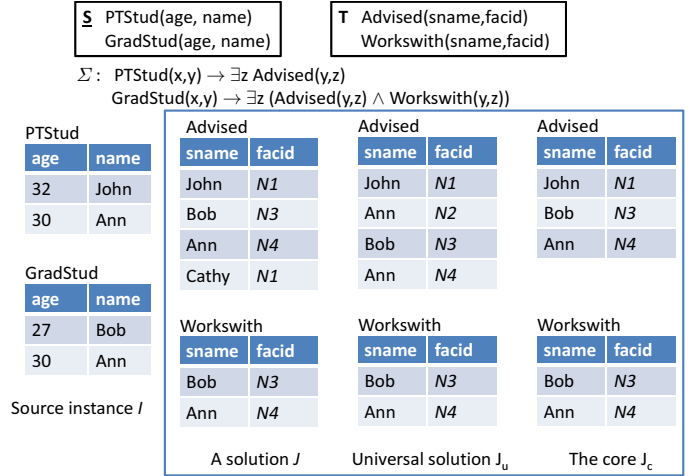
Figure 1: An example of a schema mapping \mathcal{M} = (\mathcal{S}, \mathcal{T}, \Sigma) , a source instance I , a solution J for I , a universal solution J_u for I , and the core J_c for I .
