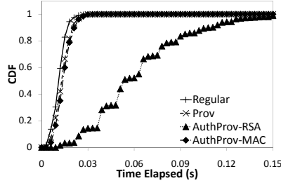
Fig. 11. CDF of packet delivery latency for traffic traceback on the local cluster.
