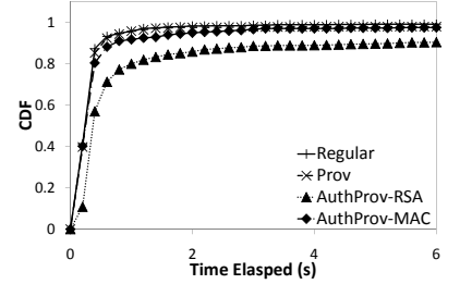
Fig. 12. CDF of packet delivery latency for traffic traceback on PlanetLab.
