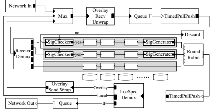
Fig. 1. Dataflow execution plan for a single node.
